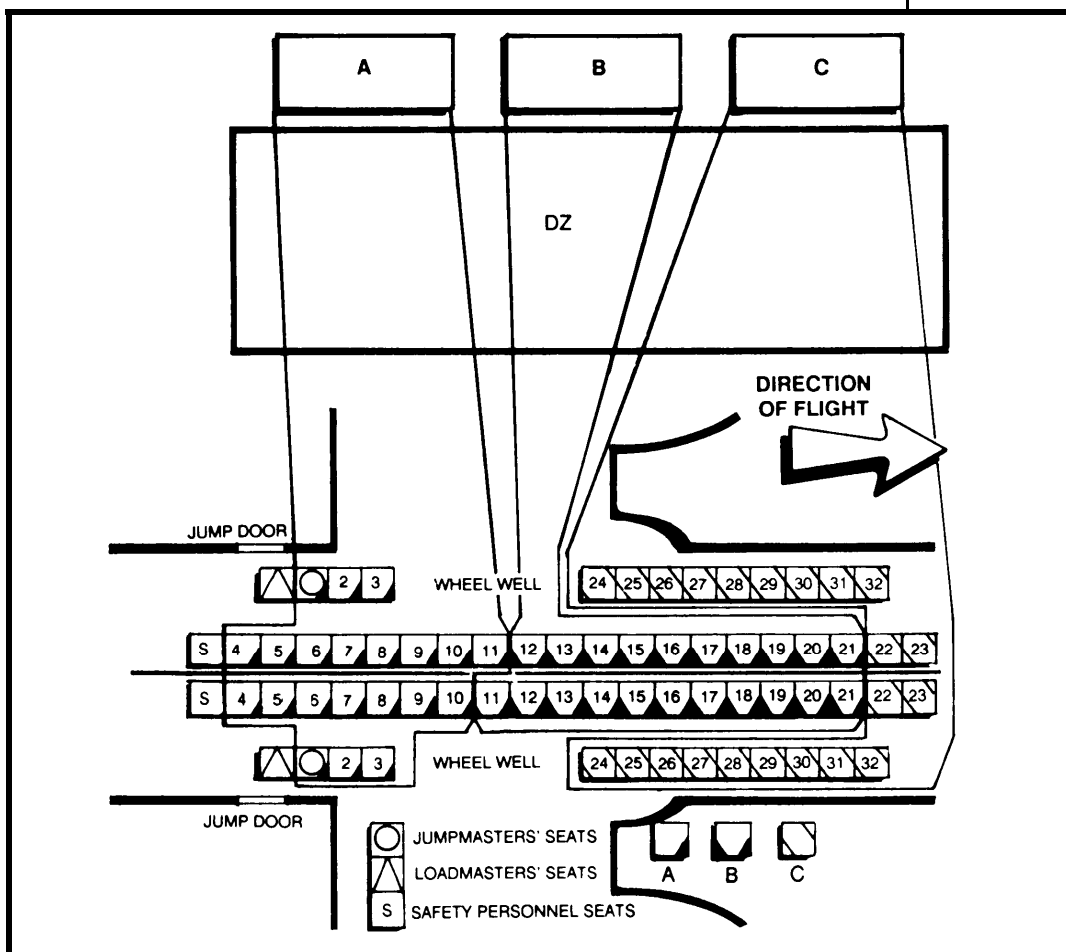
Figure 5-4. Cross-loaded aircraft.
